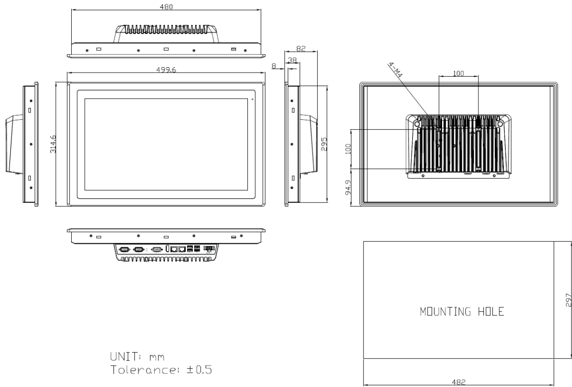
Figure 7 Dimensions of ARCHMI-S-918D P/R(H)
