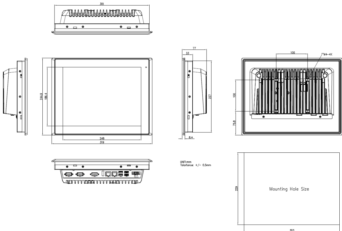
Figure 2 Dimensions of ARCHMI-S-912DP/R(H)
