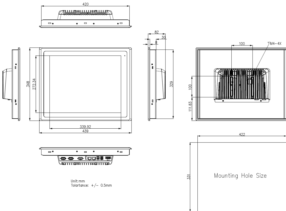
Figure 6 Dimensions of ARCHMI-S-917DP/R(H)
