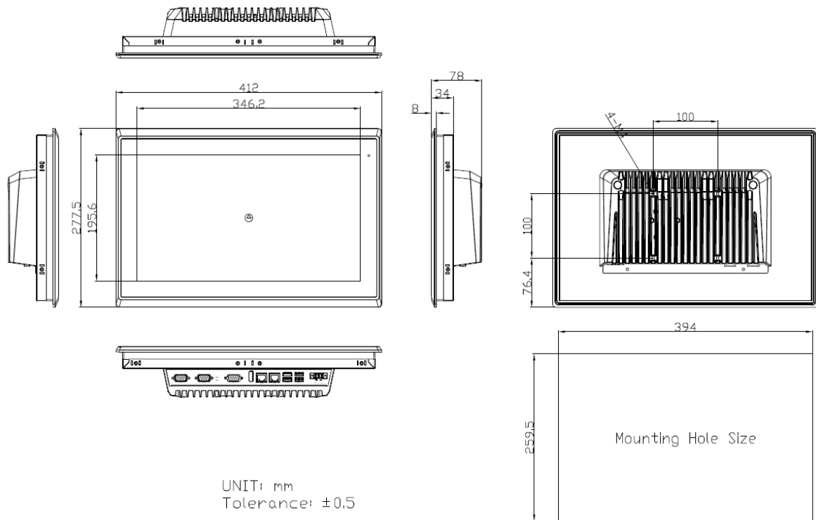
Figure 5 Dimensions of ARCHMI-S-916DP/R(H)
