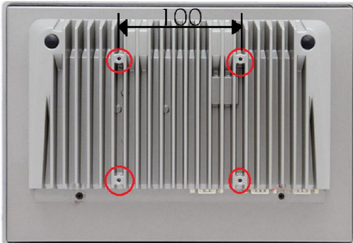
Figure 13 ARCHMI-S-9XXD VESA Mounting
