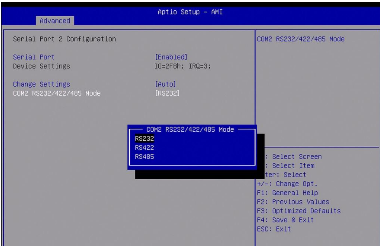
Com2 RS232/422/485 Mode
