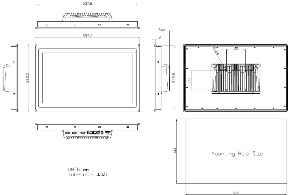
Figure 9 Dimensions of ARCHMI-S-921DP/R(H)
