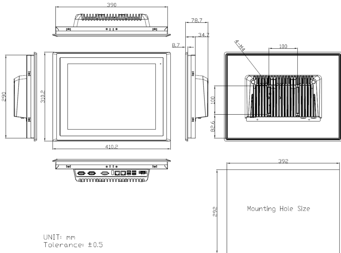
Figure 4 Dimensions of ARCHMI-S-915DP/R(H)
