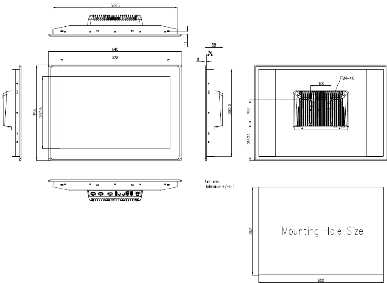
Figure 10 Dimensions of ARCHMI-S-924DP(H)
