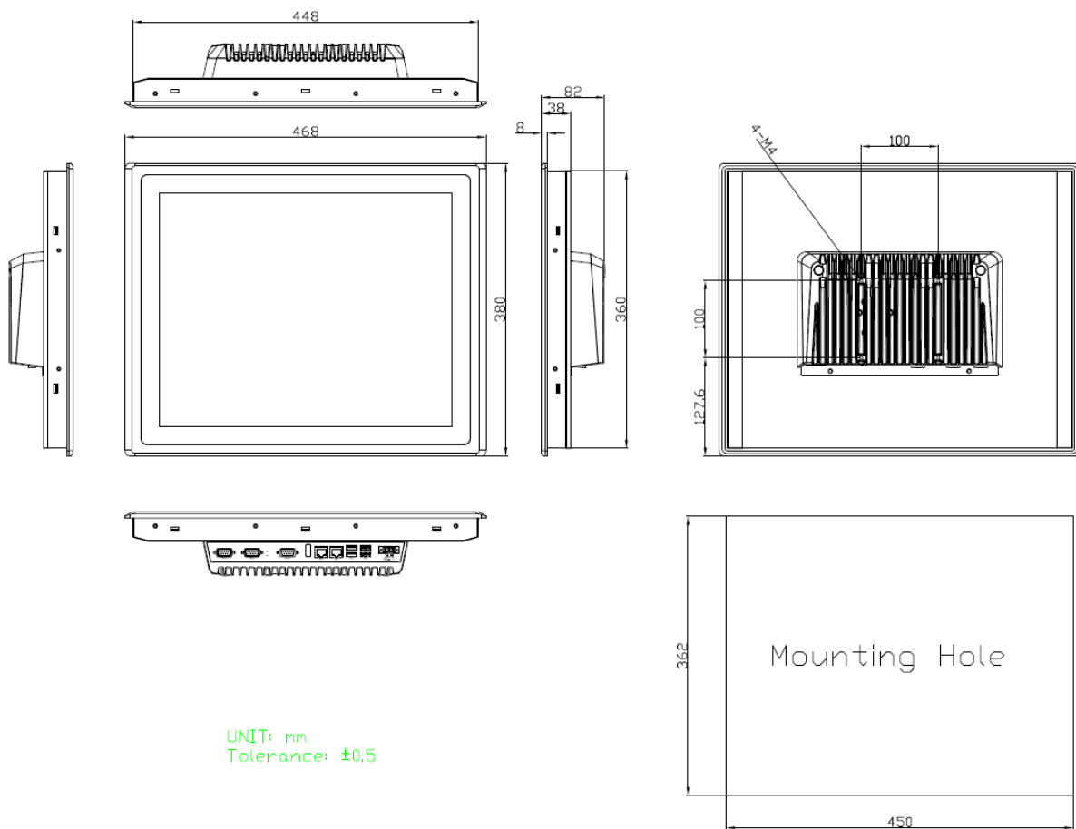
Figure 8 Dimensions of ARCHMI-S-919D P/R(H)
