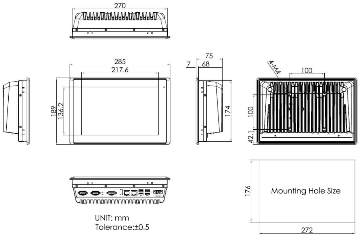
Figure 1 Dimensions of ARCHMI-S-910DP/R(H)
