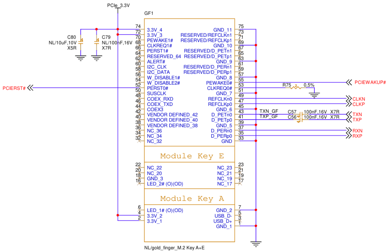
Figure 3: M.2 A-E Key Pin Define
