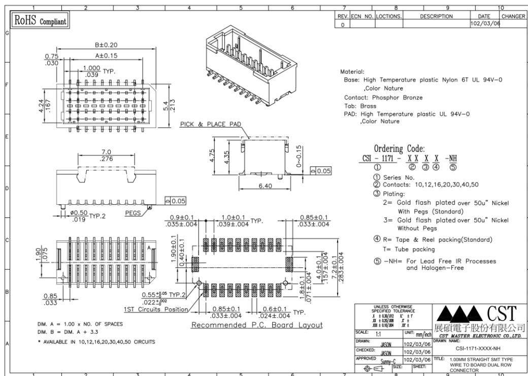
Figure 5: Wire to Board SMD 2*10P 180D Connector Drawing (CN2)
