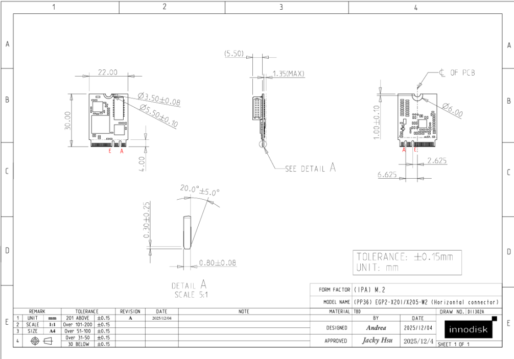
Figure 7: EGP2-X205-W2 Drawing
