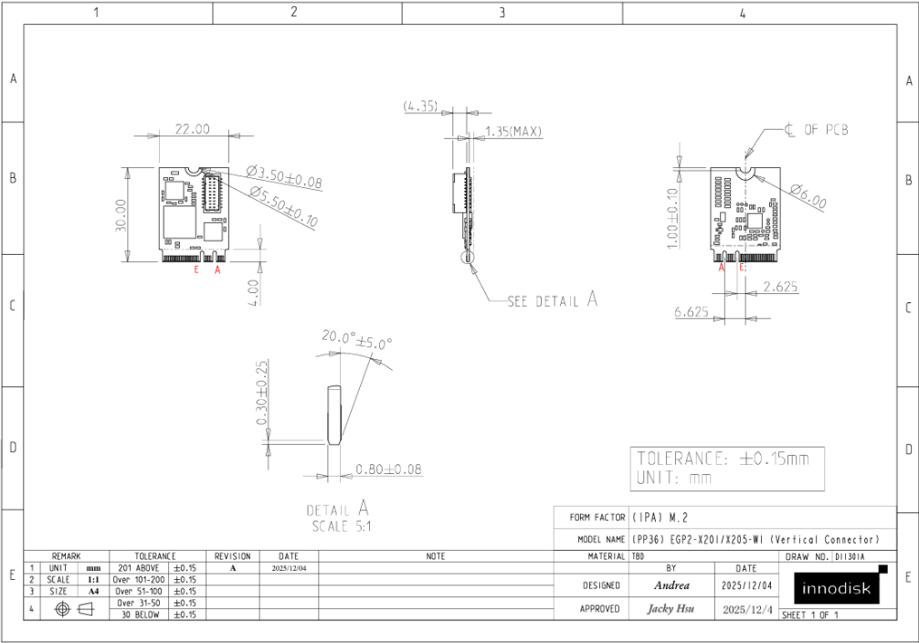
Figure 6: EGP2-X205-W1 Drawing
