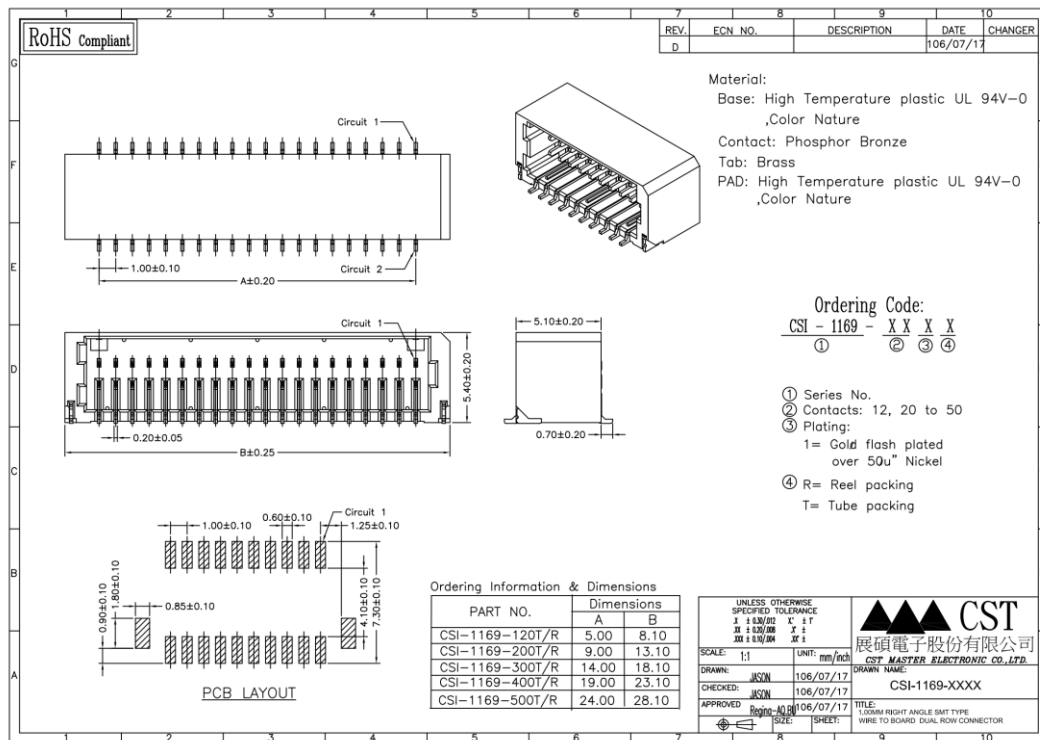
Figure 4: Wire to Board SMD 2*10P 90D Connector Drawing (CN1)
